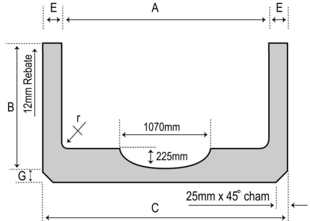
SC SUPERSIZE U-SHAP DRAIN WITH DRY WEATHER FLOW SECTION
