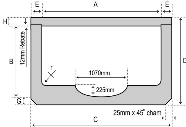
SC LARGE PRECAST R. C. BOX CULVERTS Incorporated with a Dry Weather Flow Section
