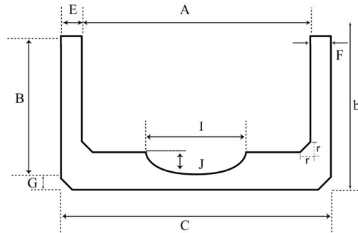
SC U-SHAPE DRAIN WITH A DRY WEATHER FLOW
