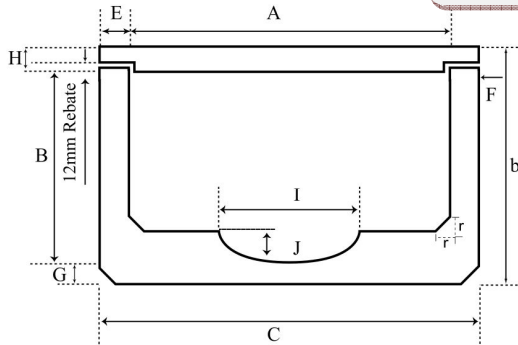
R.C BOX CULVERT WITH A DRY WEATHER FLOW
